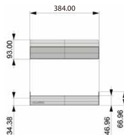
1. Grease Tray
