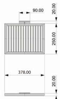
3. Resting Grill
